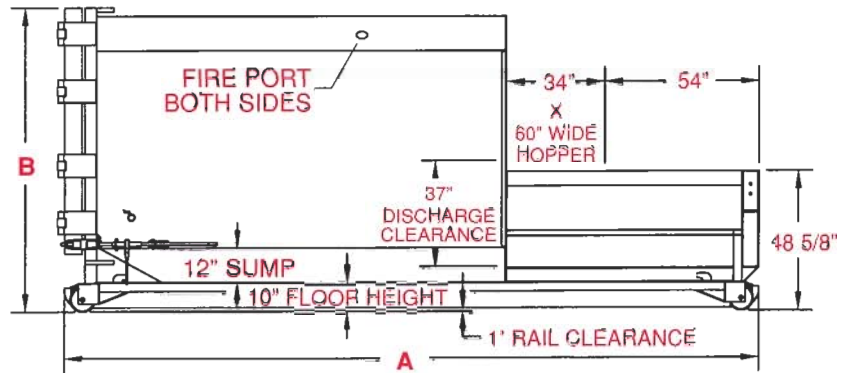
Compactor-Left Hand Side Shown-Front and Back Wheels (4) 73 1/2" O.D., 63 1/2" I.D.
